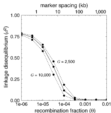
Fig. 4 LD around a variant of 50% frequency for different expansion times. Filled line, G=5,000 ; dashed lines, G=2,500 or G=10,000 , as marked.
